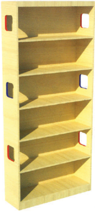
OD-01LIB LIBRARY SHELF ■ ■ Size: W812xD305xH2082mm
